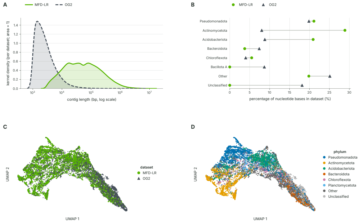
Figure 1. Characterisation of the LOAM pre-training corpus
