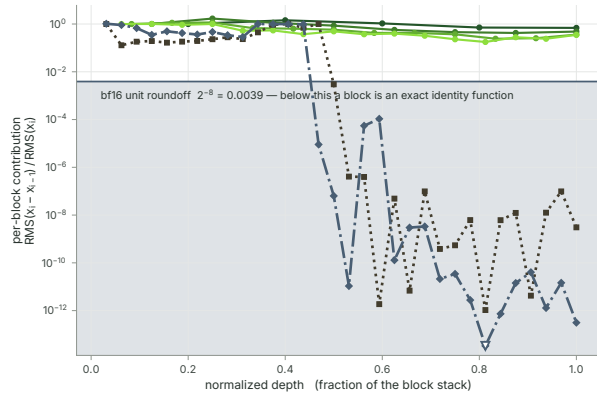
Figure S1. Layer collapse and health monitoring.
