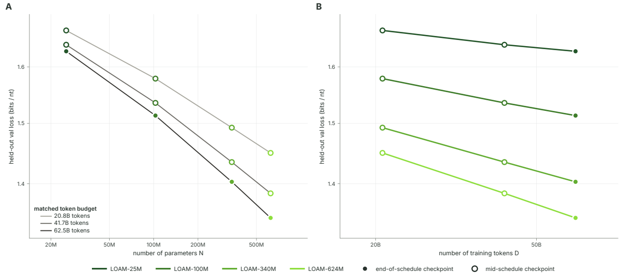
Figure S2. LOAM validation loss scales with model size and training tokens
