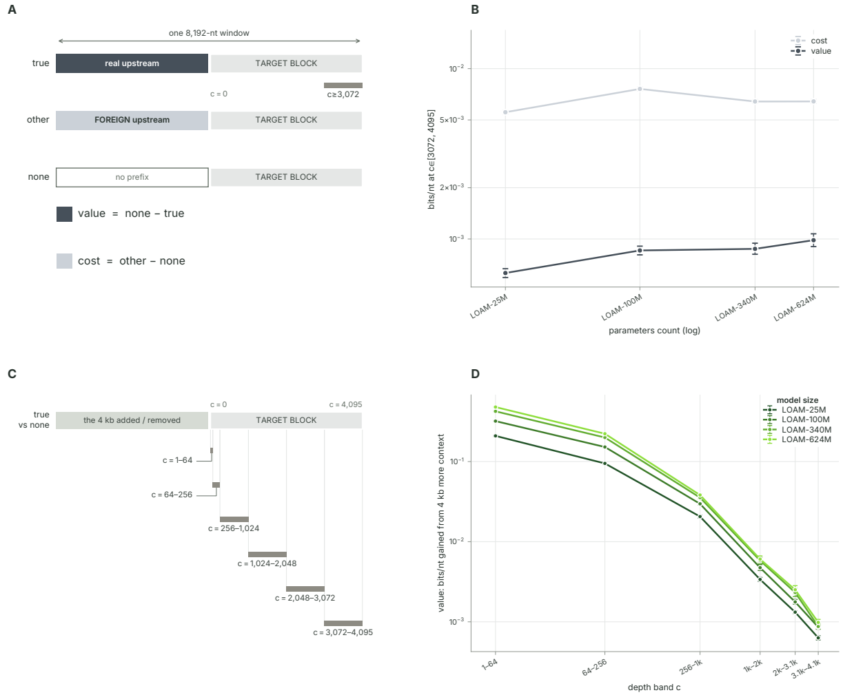
Figure 3. LOAM models use distal genomic context
