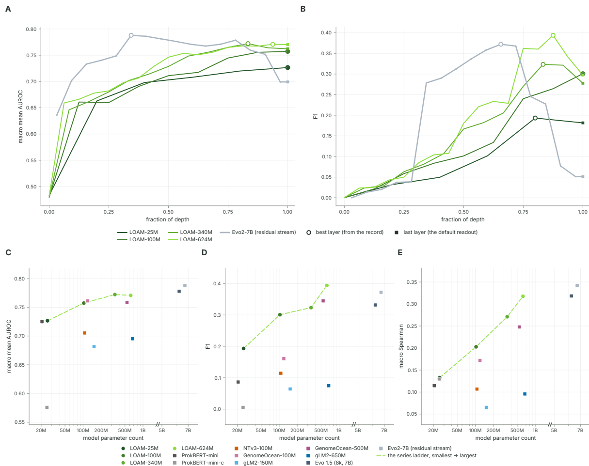
Figure 4. Layer-wise representations and performance across biological benchmarks
