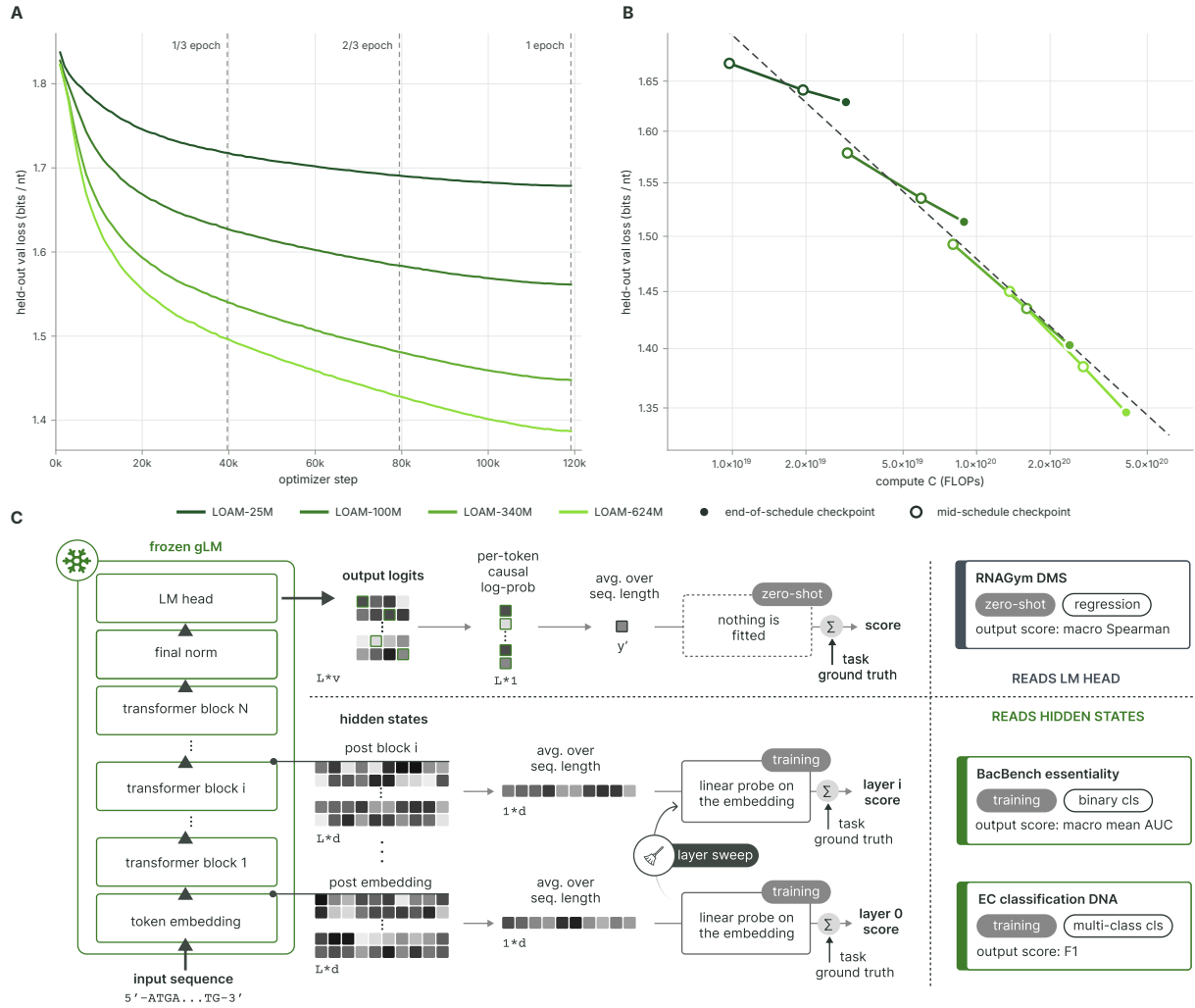
Figure 2. LOAM training dynamics and evaluation framework
